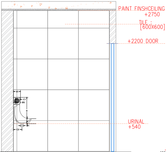
SECTIONAL ELEVATION - WALL B
