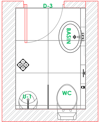
TOILET: FURNITURE LAYOUT
