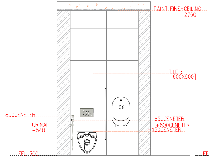
SECTIONAL ELEVATION - WALL A
