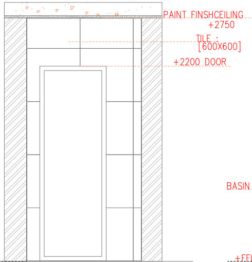
SECTIONAL ELEVATION - WALL C
