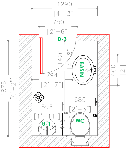
TOILET: FIXTURES LAYOUT
