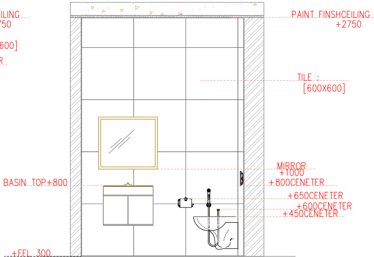
SECTIONAL ELEVATION - WALL D
